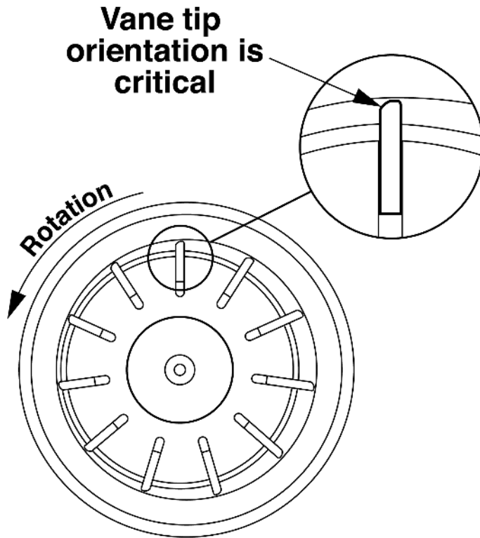
Pump body viewed from cover side
