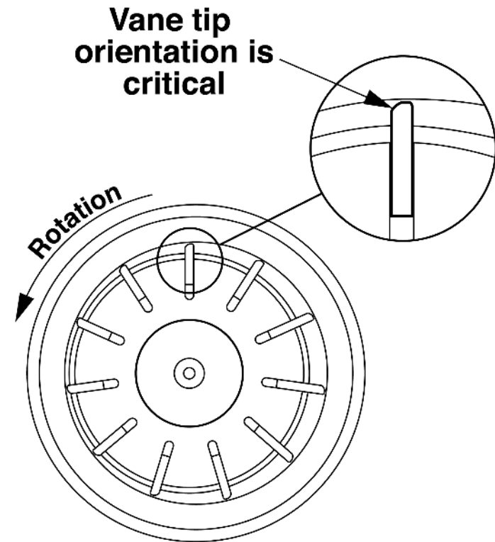
Pump body viewed from cover side
